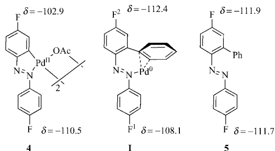
Scheme 5. 19 F NMR features of 4 , I and 5 . All the chemical shifts are given for the species in methanol.
