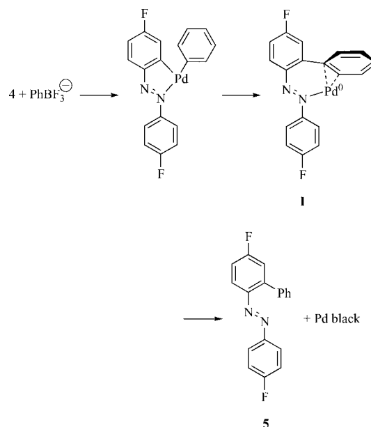
Scheme 6. Reaction of 4 with phenyltri-fluoroborate generates Pd 0 complex I , which slowly decomposes to 5 .
