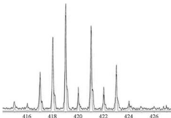
Figure 2. Experimental (solid line) and simulated (dotted line) HRMS(–) spectrum of I as its fluoride adduct. The error between simulated and observed isotopic patterns is –1.72 ppm.
