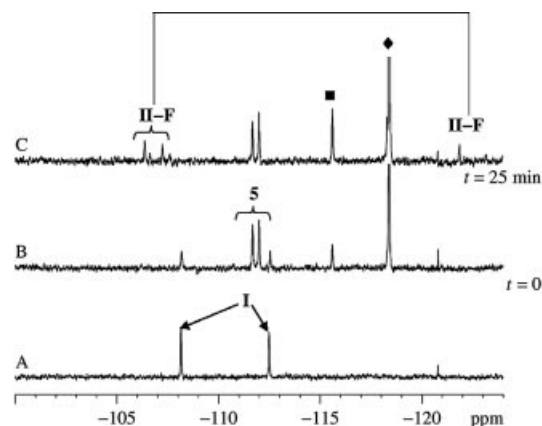
Figure 5. Reaction of 4 with excess KPhBF 3 and p -FC 6 H 4 N 2 BF 4 . A: 4 /KPhBF 3 ; B: immediately after addition of p -FC 6 H 4 N 2 BF 4 ; C: after 25 min. ■ = 4,4'-difluorobiphenyl; ◆ = 4-fluorobiphenyl. Pd/diazonium/KPhBF 3 molar ratio of 1:15:18.
