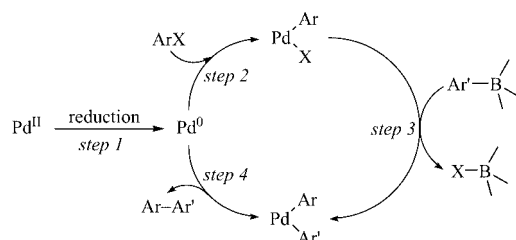
Scheme 3. General catalytic cycle for the Suzuki cross-coupling reaction leading to biaryls.
