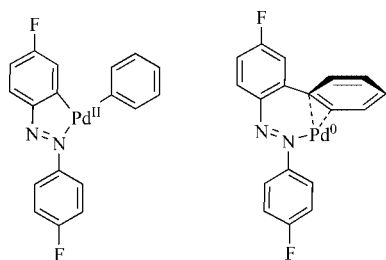
Scheme 4. Two possible structures for species I .
