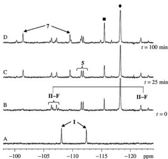
Figure 3. ^{19}\text{F} NMR monitoring of the reaction mixture of 4 /KPhBF 3 and p -FC 6 H 4 N 2 BF 4 in methanol. A: 4 /KPhBF 3 ; B: immediately after addition of p -FC 6 H 4 N 2 BF 4 ; C and D: after 25 and 100 min, respectively. ■ = 4,4'-difluorobiphenyl; ◆ = 4-fluorobiphenyl. Pd/diazonium/KPhBF 3 molar ratio of 1:18:15.
