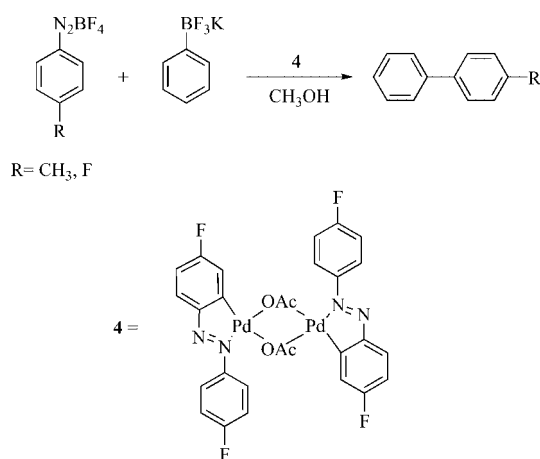
Scheme 2. Cross-coupling reaction with a fluorinated substrate and precatalyst 4 .
