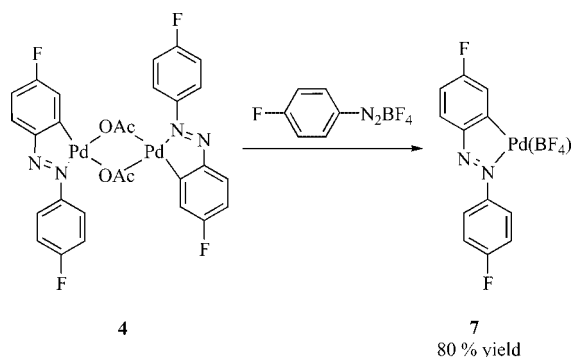
Scheme 8. Formation of complex 7 .
