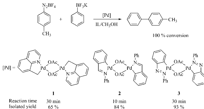
Scheme 1. Examples of highly active palladacycles for the cross-coupling reaction. [3] IL = 1- n -butyl-3-methylimidazolium tetrafluoroborate.
