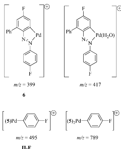
Scheme 7. Pd II species detected by HRMS(+) in the reaction mixture of 4 /KPhBF 3 after the addition of p -FC 6 H 4 N 2 BF 4 .
