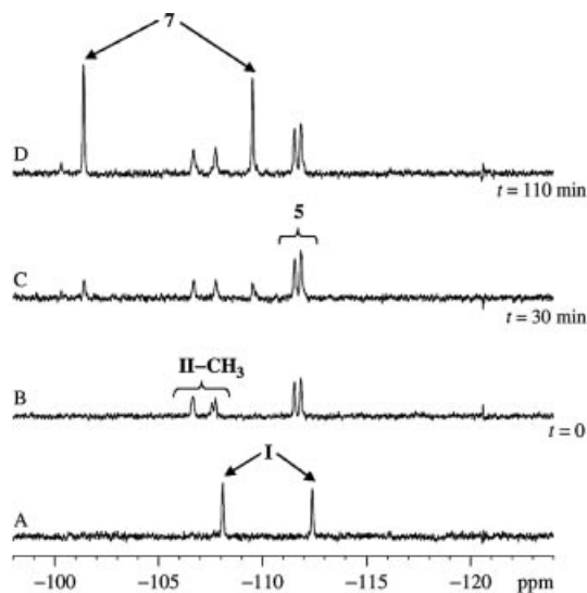
Figure 4. ^{19}\text{F} NMR monitoring of the reaction mixture of 4 /KPhBF 3 and p -CH 3 C 6 H 4 N 2 BF 4 in methanol. A: 4 /KPhBF 3 ; B: immediately after addition of p -CH 3 C 6 H 4 N 2 BF 4 ; C and D: after 30 and 110 min, respectively. Pd/diazonium/KPhBF 3 molar ratio of 1:18:15.
