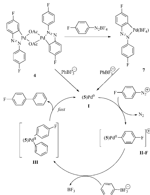
Scheme 9. Proposed catalytic cycle for the palladium-catalyzed cross-coupling of diazonium salts with aryltrifluoroborates.
