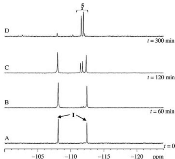
Figure 1. 19 F NMR spectroscopic monitoring of reaction mixtures of 4 and KPhBF 3 in methanol as a function of time (Pd:KPhBF 3 = 1:15 mol/mol).
